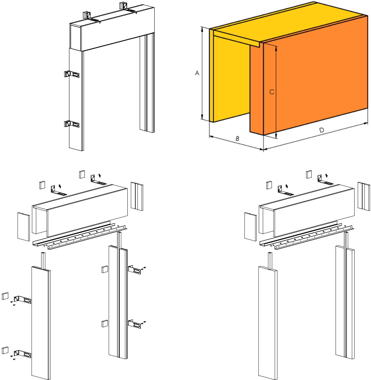
Box: ISOTRA PB-IS 2-01835-XXXX-... surround: PIO - Purenit insulation jambs
